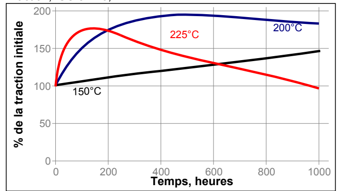
Traction, ISO 527-3,
