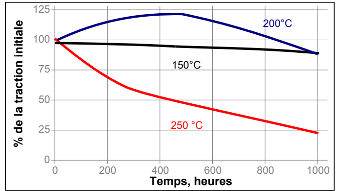
Traction, ISO 527-3,
